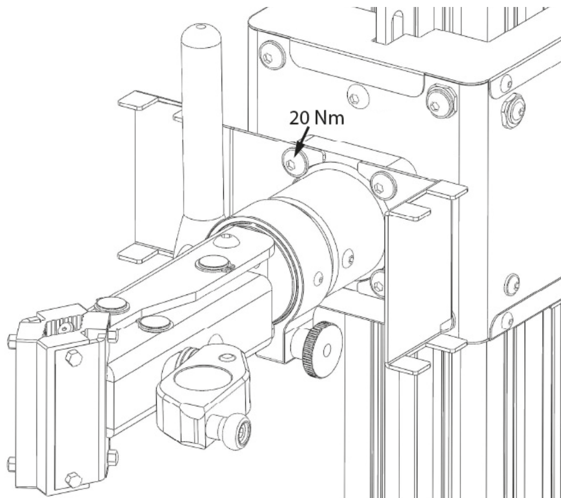
Figur 2: Holderens monteringsposition
