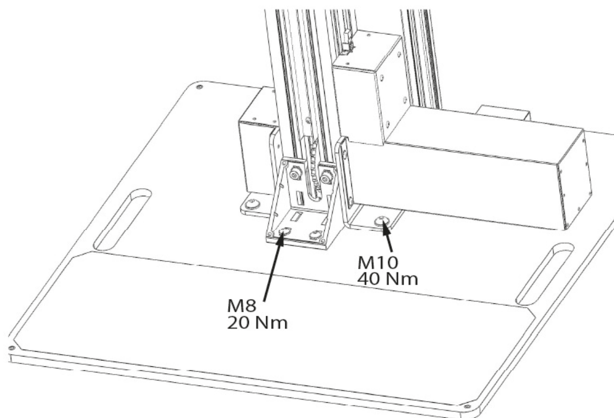
Figur 3: Standmonteringsskruer
